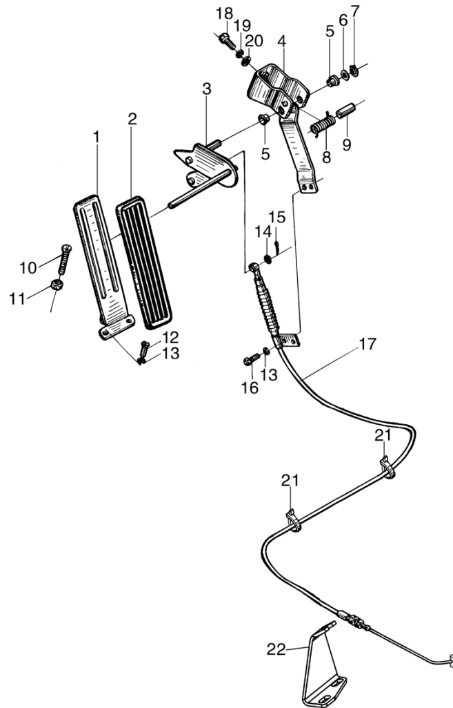
图 11 油门操纵总成 Fig.11 Throttle control assy
