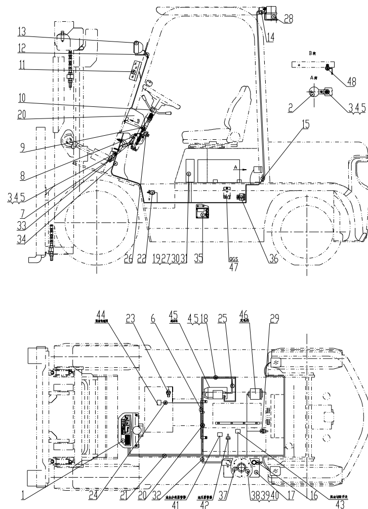
Fig.21 Electrical system (OPS System)
