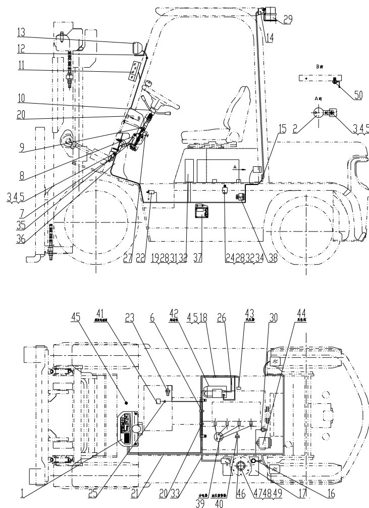
Fig.20 Electrical system (OPS System)
