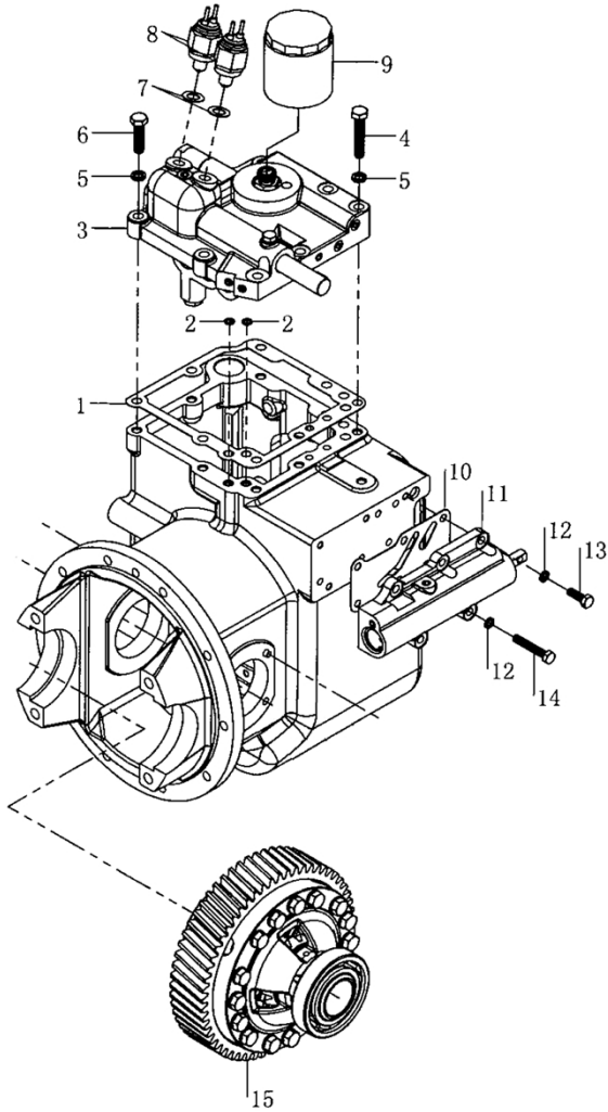
inching valve (tor-con type) SHAOXIN
