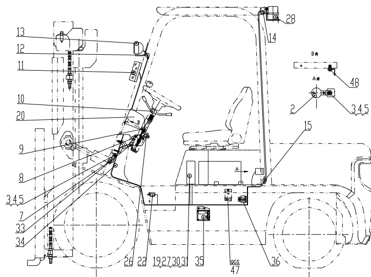
Fig.21 Electrical system (OPS System)
