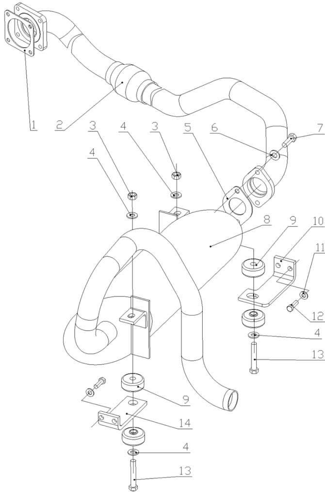
Fig.27 Exhaust system
