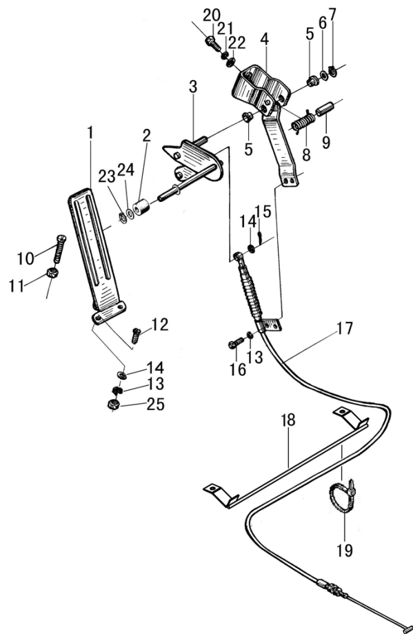
图 10-1 油门操纵总成 Fig.10-1 Throttle control assy
