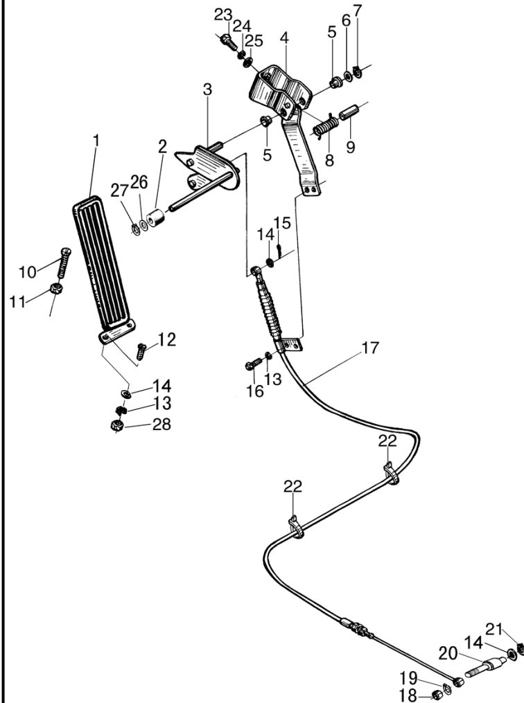
图 12-1 油门操纵总成 Fig.12-1 Throttle control assy
