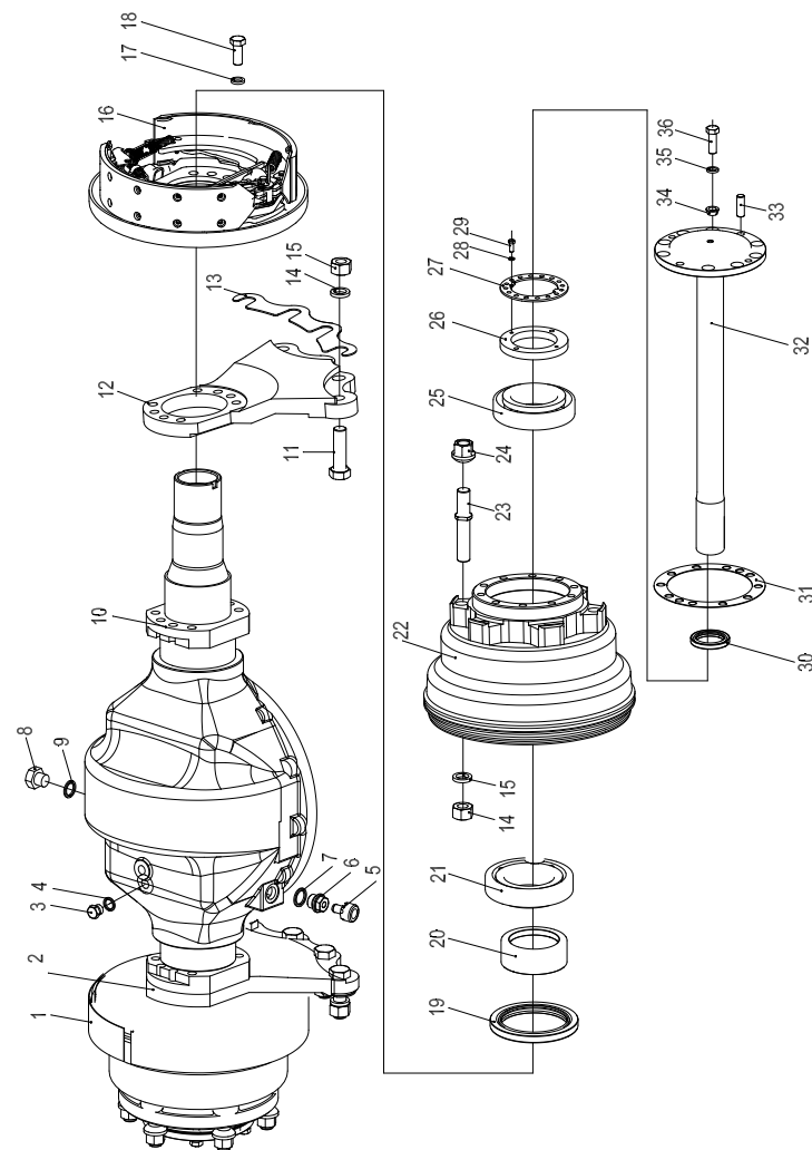
图 13-1 驱动桥 Fig.13-1 Drive axle
