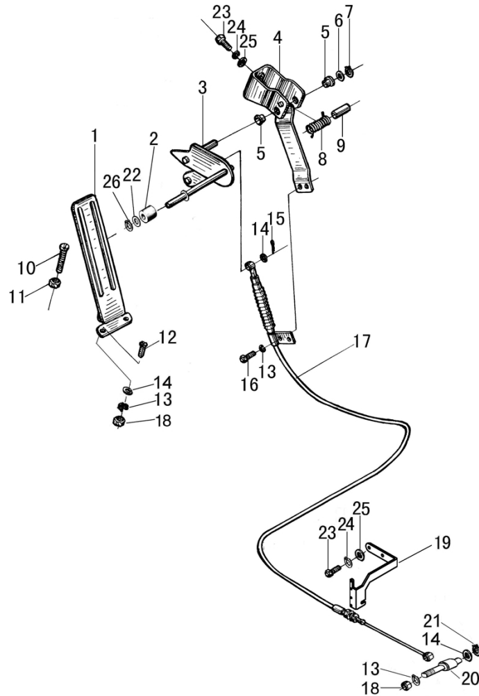
图 9-1 油门操纵总成 Fig.9-1 Throttle control assy ≥2014-02-01
