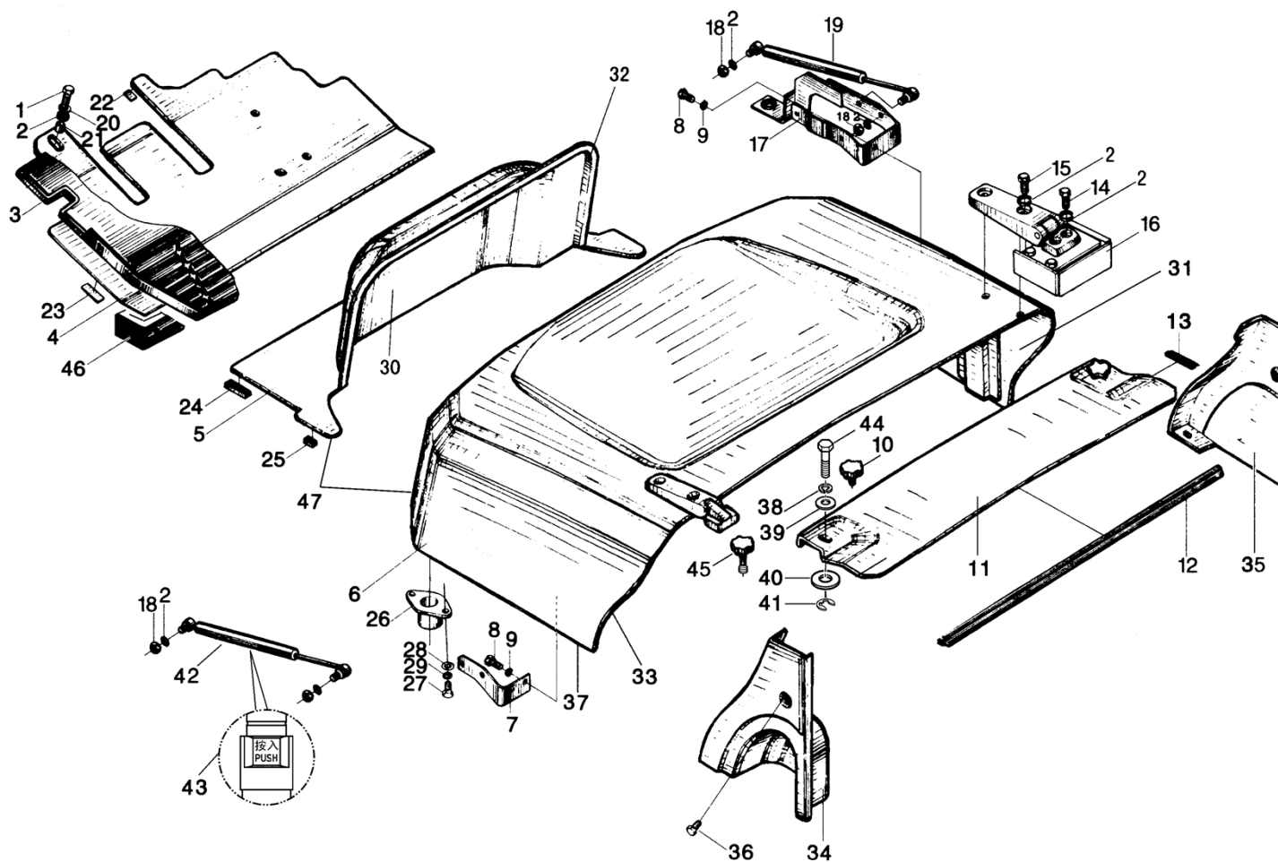
Fig.6 Hood and floor board assy( I )
