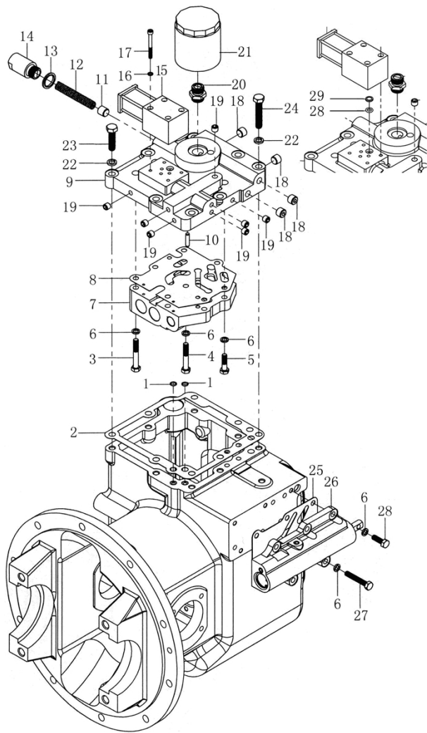
图 20 盖、控制阀、微动阀（液力式）绍兴 Fig.20 Cover control valve & inching valve (tor-con type) SHAOXIN
