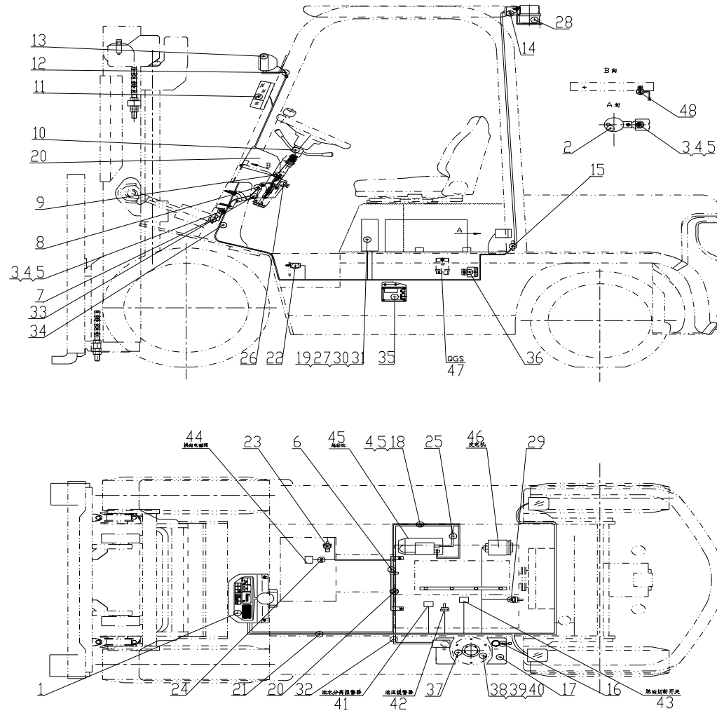
Fig.21 Electrical system (OPS System)
