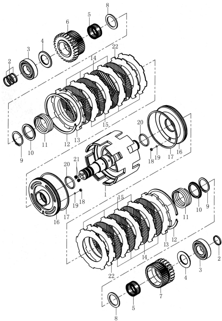
Fig.19 Hydraulic clutch(tor-con type)
