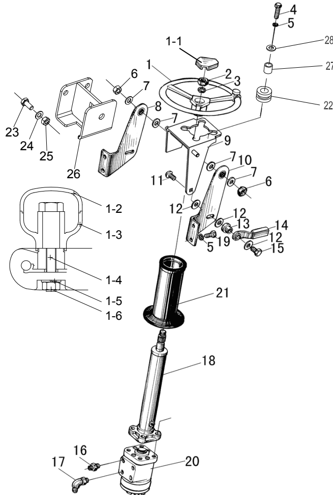
Fig.5-1 Steering device(Shock absorption)
