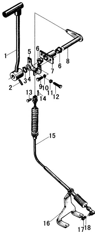
Fig. 17 Change over control assy
