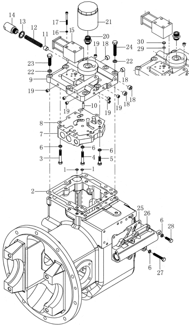
Fig.20 Cover control valve & inching valve (tor-con type) SHAOXIN
