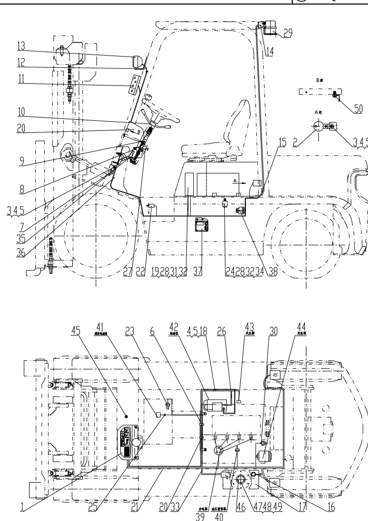
Fig.20 Electrical system (OPS System)
