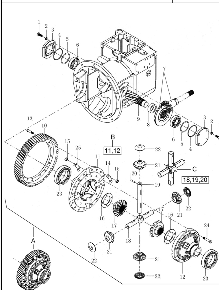
图 22 减速器和差速器 (绍兴) Fig.22 Reduction & differential (ShaoXin)
