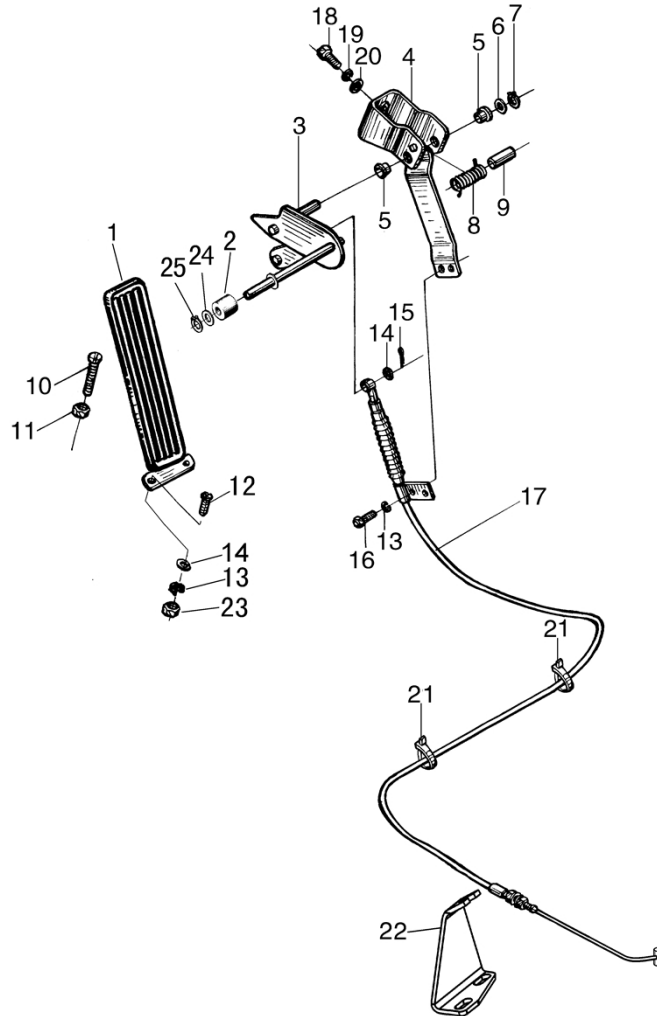
图 11-1 油门操纵总成 Fig.11-1 Throttle control assy
