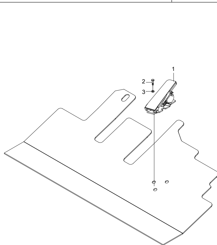
图 13 油门操纵总成(电子) Fig.13 Throttle control assy (Electron)
