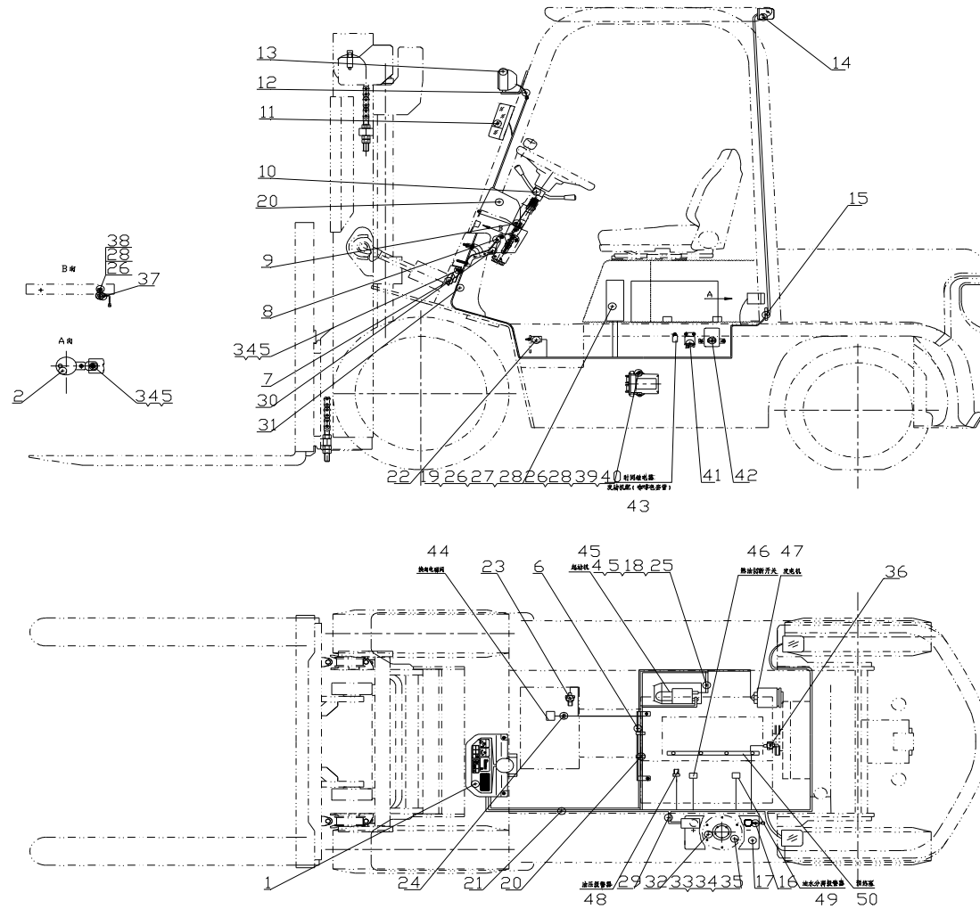
Fig.22 Electrical system (OPS System)
