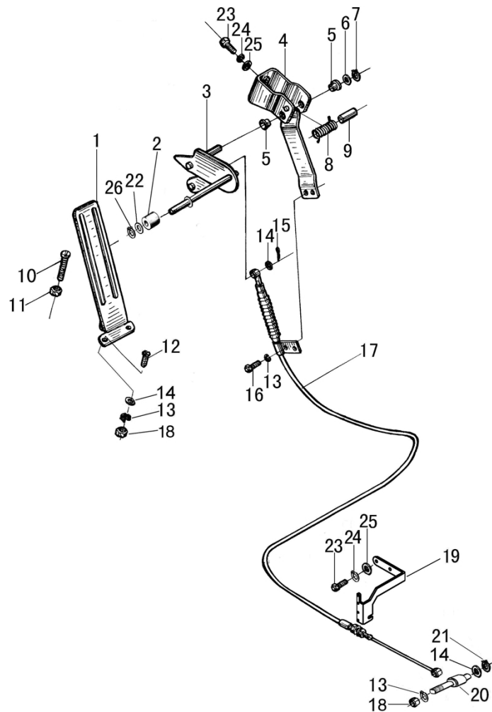
图 9-1 油门操纵总成 Fig.9-1 Throttle control assy
